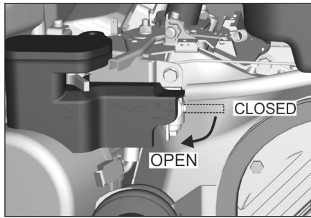
Figure: Open fuel cock (petrol/gas engine)
