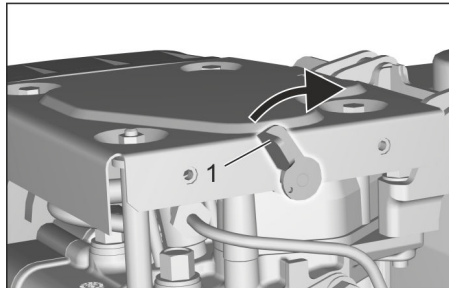
Figure: Decompression lever (diesel engine)
