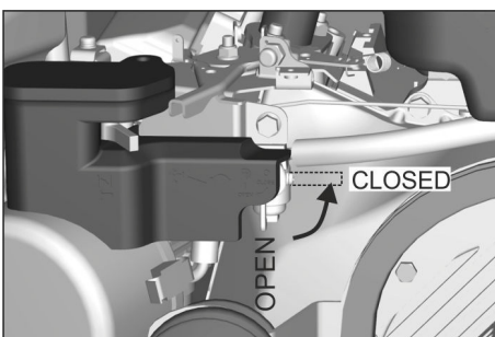
Figure: Close fuel cock (petrol engine)
