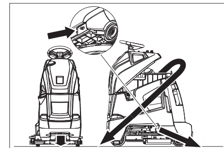
Fastening points
