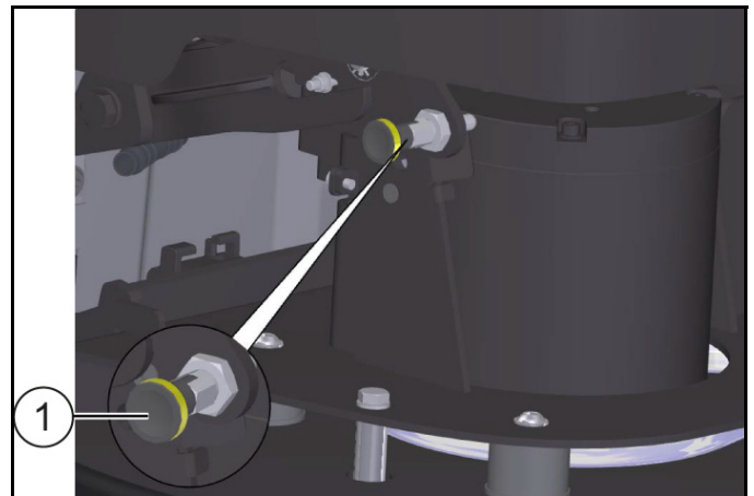
① Locking pin suspension
