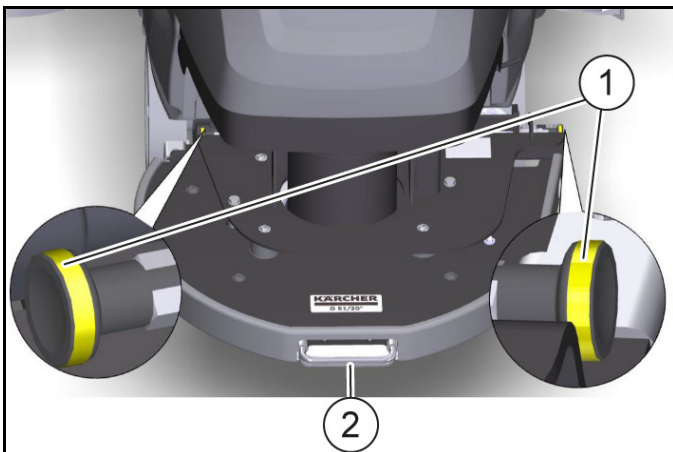
① Push rod locking pin ② Handle
