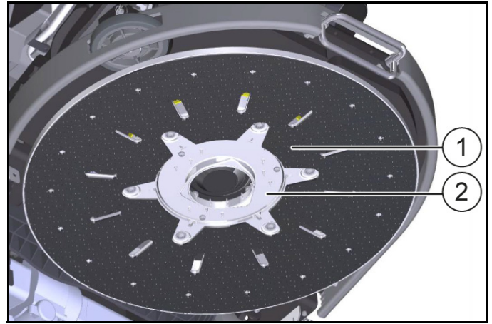
① Pad drive board ② Centre lock
