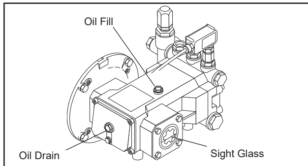
Figure 10 - Pump Lubrication
