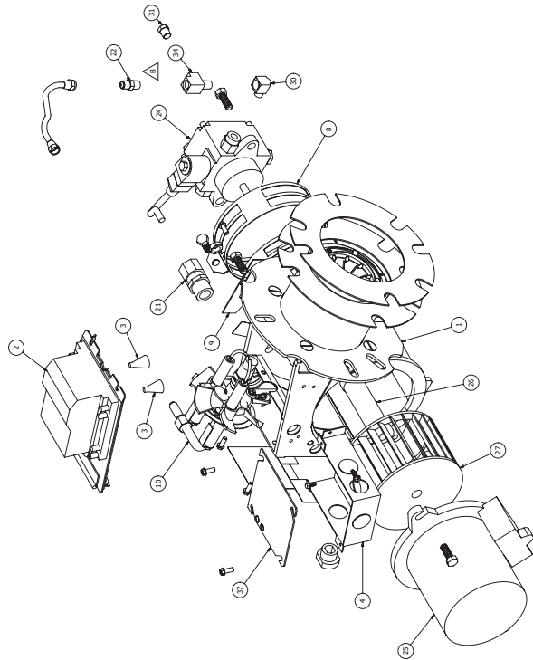
EXPLODED VIEW
