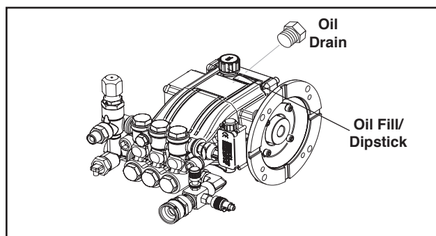
Figure 7 - Pump Lubrication
