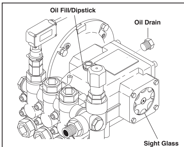
Figure 6 - Pump Lubrication
